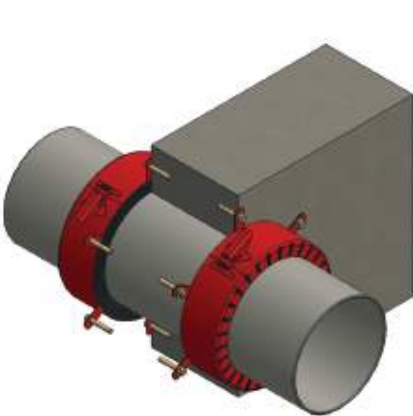
Fire Collar - In Wall
